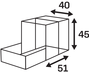
Assembled Dimensions
