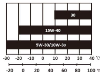
ENVIRONMENT TEMPERATURE
