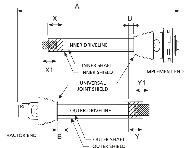
Figure 3 - Driveline Shortening
