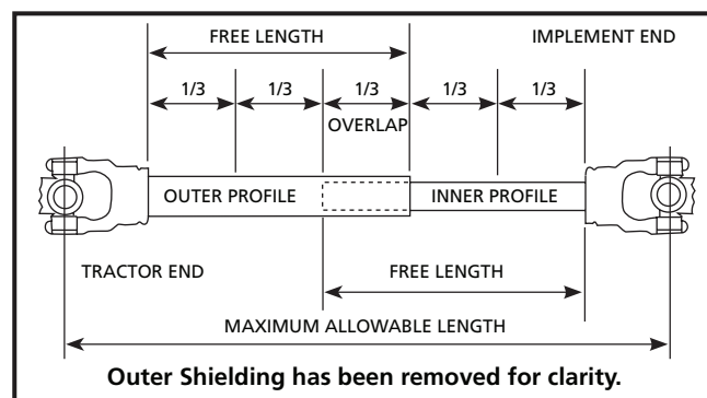
Figure 4 - Driveline Maximum Extended Length
