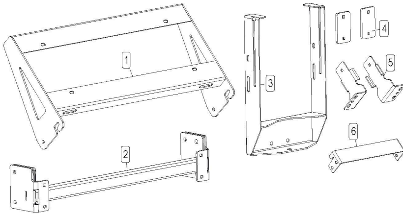
Contents of BB ZT Mount Kit #5283868
