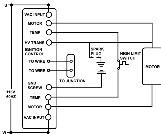
SCHEMATIC DIAGRAM
