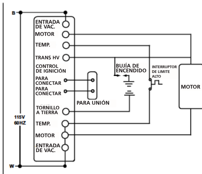
SCHEMATIC DIAGRAM
