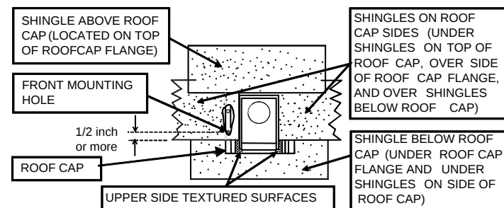
Figure 2. Shingle Placement
