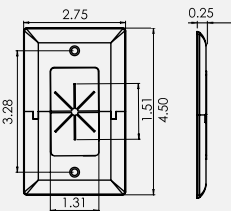
1-Gang Flexible Split plate
