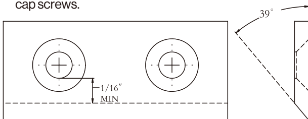
Fig.14 - Chipper knife minimum cutting edge EN
