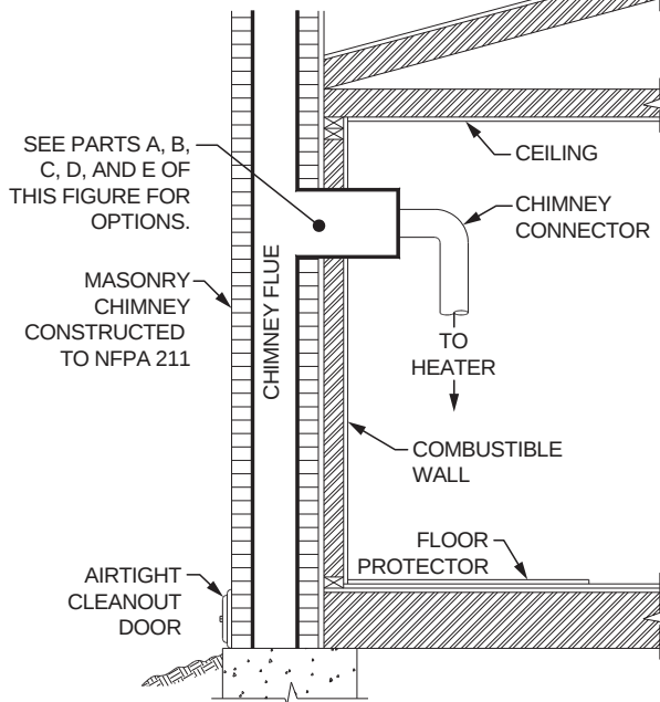
CONNECTION OF CHIMNEY CONNECTOR TO A MASONRY CHIMNEY THROUGH A COMBUSTIBLE WALL
