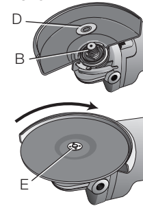
1/4" WHEELS (6.35 mm)
