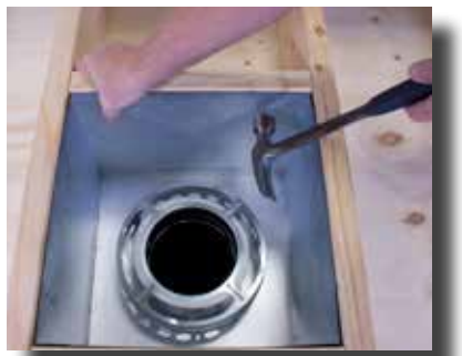
3. Nail the chimney support box to the framed opening from above. Use at least two 8 penny nails on each side.
