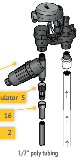
RBC 8000 Battery Powered Timer with 3/4" Anti-Siphon Valve
