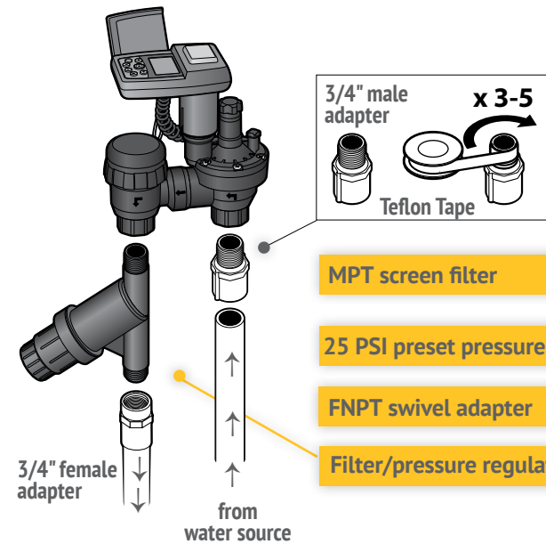
ECO1 ASV.075 Solar Powered Timer with 3/4" Anti-Siphon Valve
