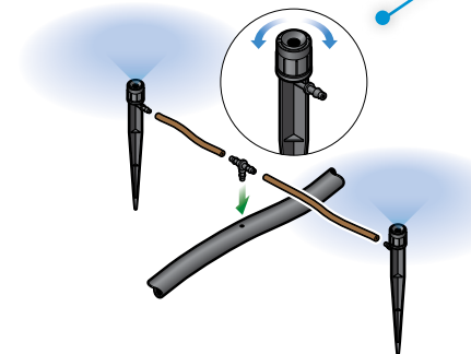
micro sprayers
