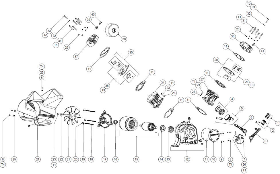
SCREW LIST - Applying torque values
