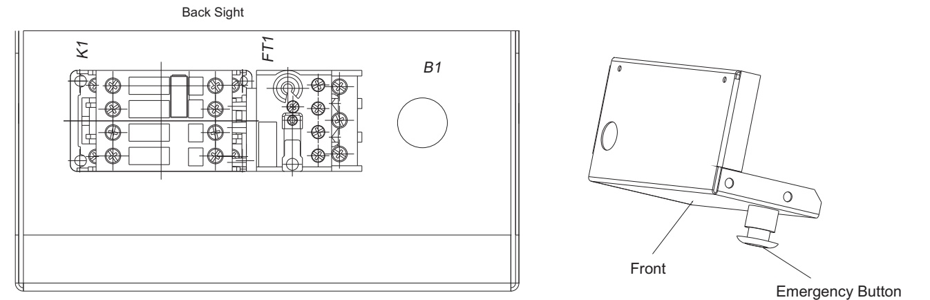
PARTS LAYOUT 5 hp - OPENED D.O.L. STARTER
