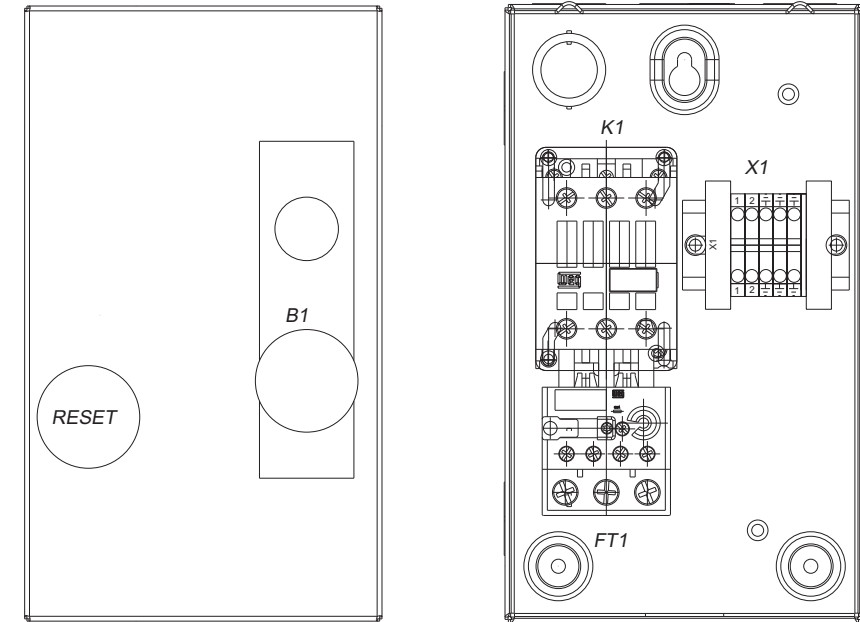
PARTS LAYOUT 5, 7.5, 10, 15 and 20 hp
