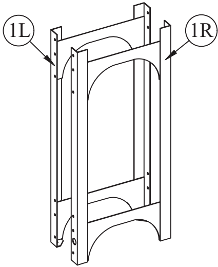
1 LEG GROUP X 2PCS
