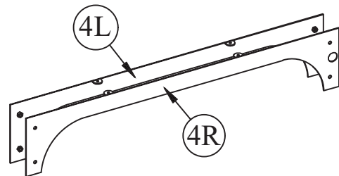
4 BOTTOM FRAME X 2PCS
