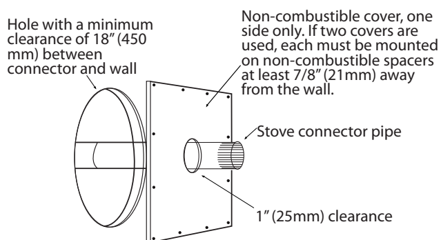
Figure 5 ONLY APPROVED CANADIAN WALL PASS THROUGH
