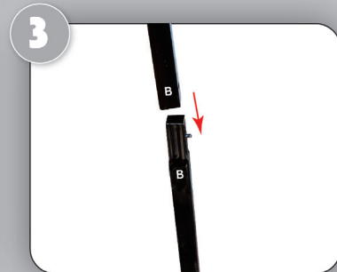
Insert and snap lock the middle left leg pole into the lower left leg pole. (Match B to B, See Figure 3)
