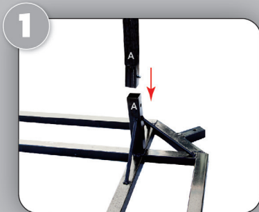
Insert and snap lock the lower left leg pole into the metal base. (Match A to A, See Figure 1)
