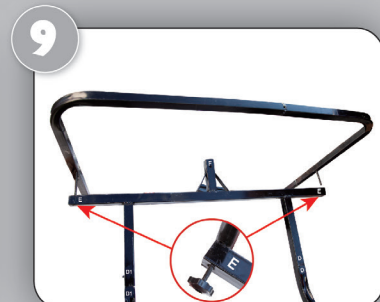
Place the waist frame on the waist support, match the hole to the hole, insert the screw and nut on the nut. (See Figure 9)
