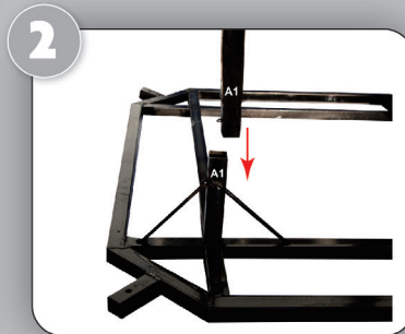
Insert and snap lock the lower right leg pole into the metal base. (Match A1 to A1, See Figure 2)
