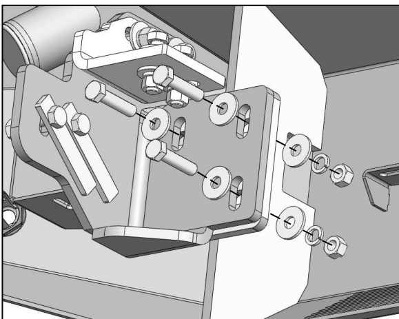
(Fig 18) Attach Bumper to Brackets
