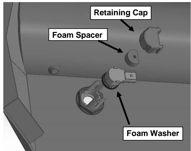
(Fig 20) Insert the sensor with seal into the sensor sleeve, followed by the foam spacer and retaining cap
