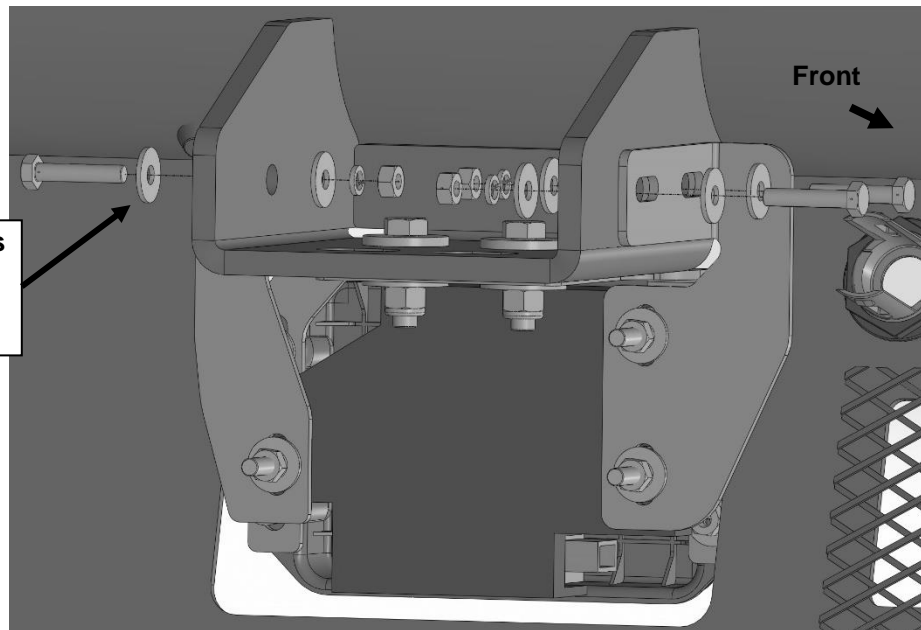
(Fig 17) Attach ACC sensor assembly to driver side tow hook bracket
