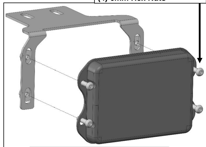
(Fig 14) Assemble ACC cover to the ACC cover bracket
