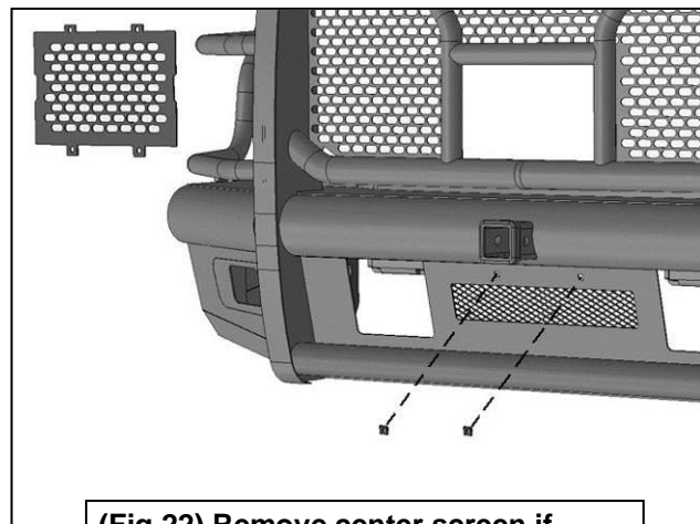
(Fig 22) Remove center screen if equipped with grille mounted camera. Install Plastic Plugs for license plate
