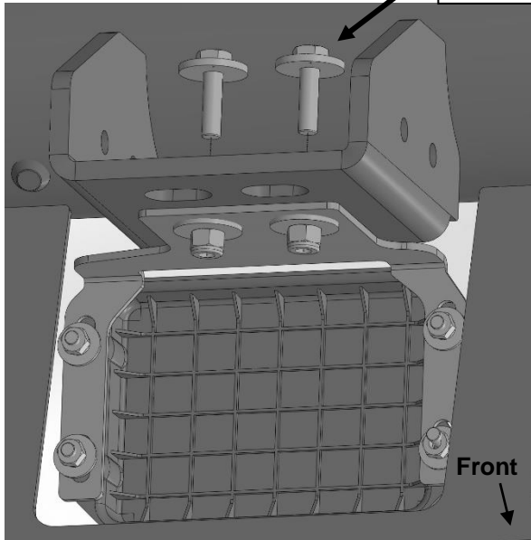
(Fig 15) Attach ACC cover assembly to the driver side tow hook bracket
