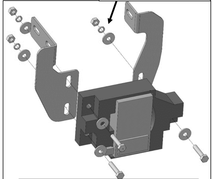
(Fig 16) Attach ACC sensor to ACC brackets
