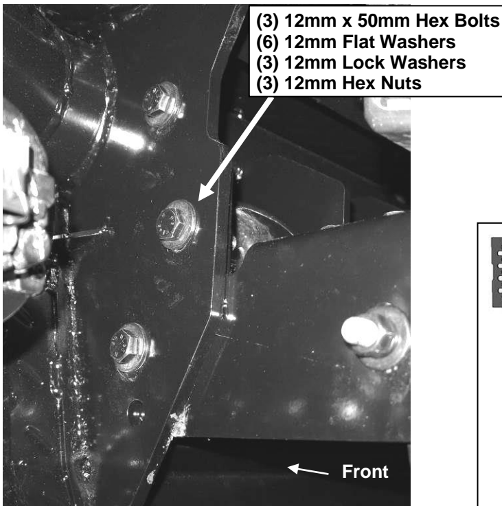
(Fig 21) Attach bumper to frame brackets
