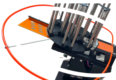
Trap Head (Circled in white, stacker poles and safety ring not yet installed)
