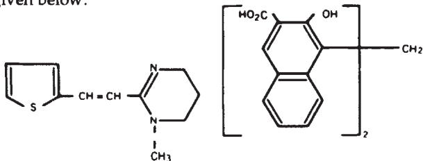
(E)-1,4,5,6-Tetrahydro-1-methyl-2-[2-thienyl] vinyl] pyrimidine 4,4' methylenebis [3-hydroxy-2-naphthoate](1:1)
