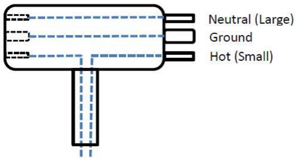
Figure 1 - Electrical Connection Schematic. The HOT / LIVE connection is interrupted and passed to the cable.
