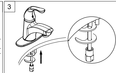
THREE HOLES INSTALLATION
