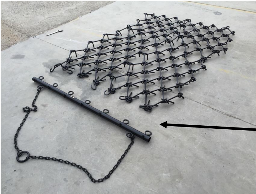
Step #5: Attach Chain Section 1 (#3) to Tow Bar (#2). See Above Photo
