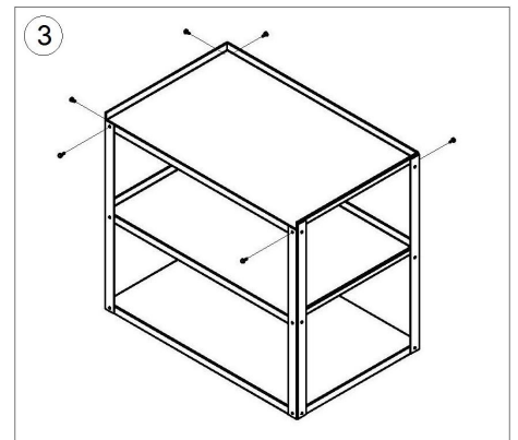
3. Fixed the top shelf with "L" supports
