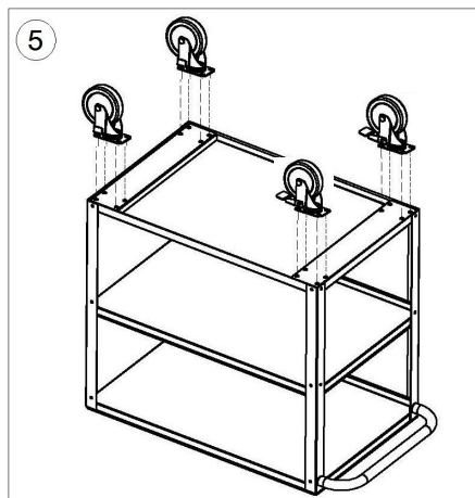
5. Turn the cart upside onto the floor, install 4pcs casters to bottom shelf
