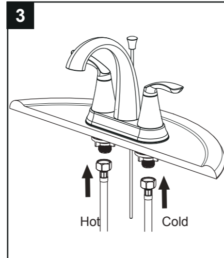
Install water inlet hoses.
