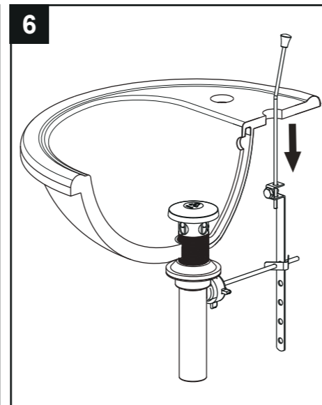
Attach the lift rod to the strap.
