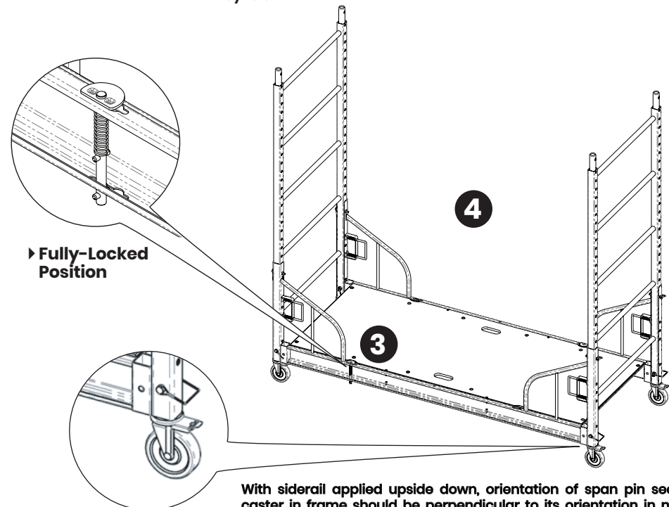
Compress Spring Downward, Tilt top Towards Large Keyhole
