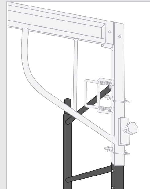
79" EXTENDED CONFIGURATION
