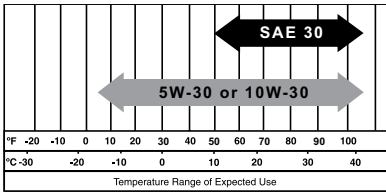
Figure 2-2. Recommended Oil
