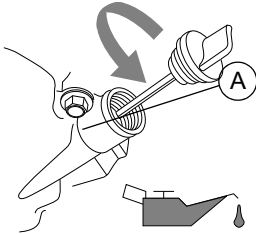
Figure 2-1. Remove Dipstick
