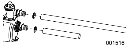
Figure 2-5. Raccord de tuyau type
