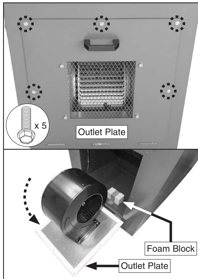
Figure 13. Location of packing material inside machine cabinet.
