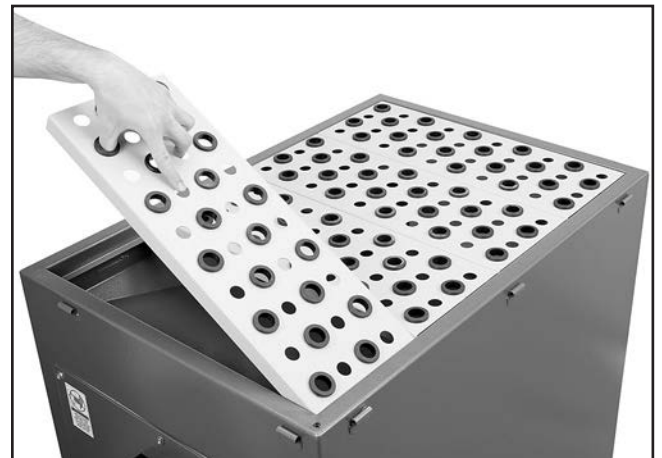
Figure 7. Installing downdraft plates.
