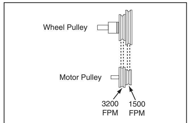
Figure 45. Drive belt position for the different speeds.
