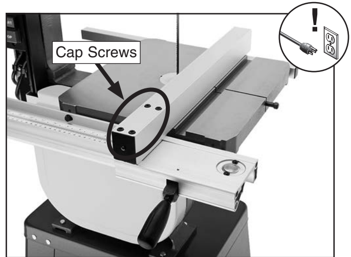
Figure 41. Location of the fence adjustment cap screws.
