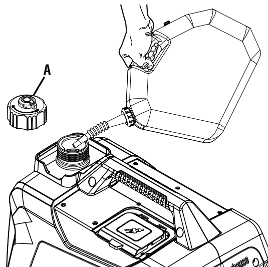
A - Vented Fuel Cap
