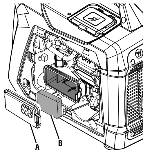
A - Air Filter Cover B - Air Filter
