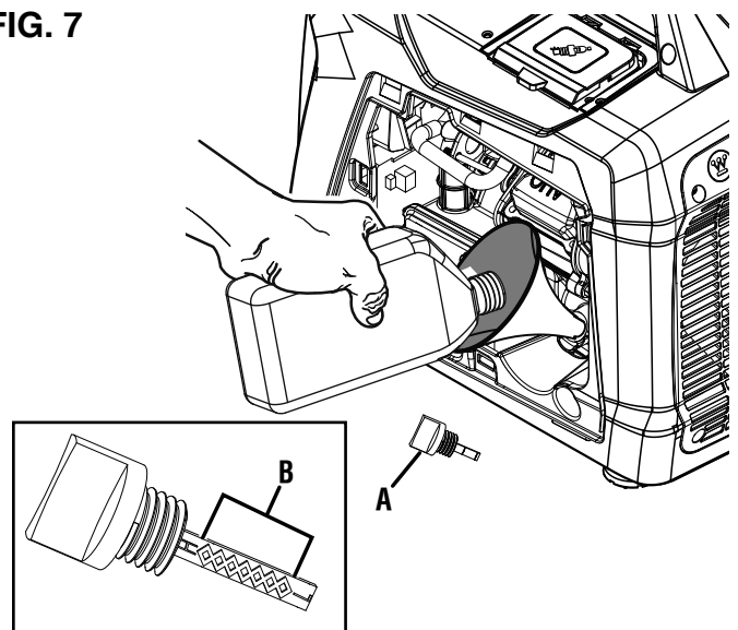
A - Oil Dipstick B - Safe Operating Range
