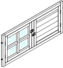
Front panel - Upper 1PC
