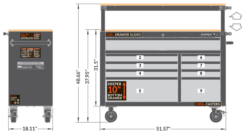
Outside dimensions and drawer numbers
