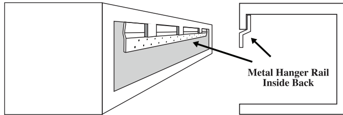
Back View of Non-Combustible Shelf
