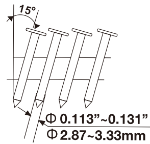
(Wire collation)
