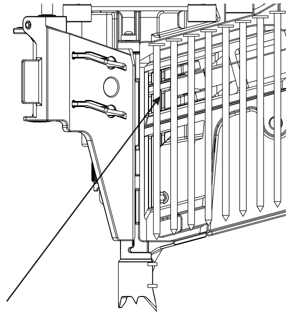
Guides(I)
