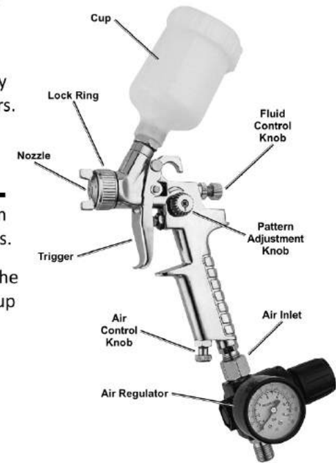
Figure C: Components & Controls
