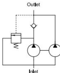
Hydraulic Schematic
