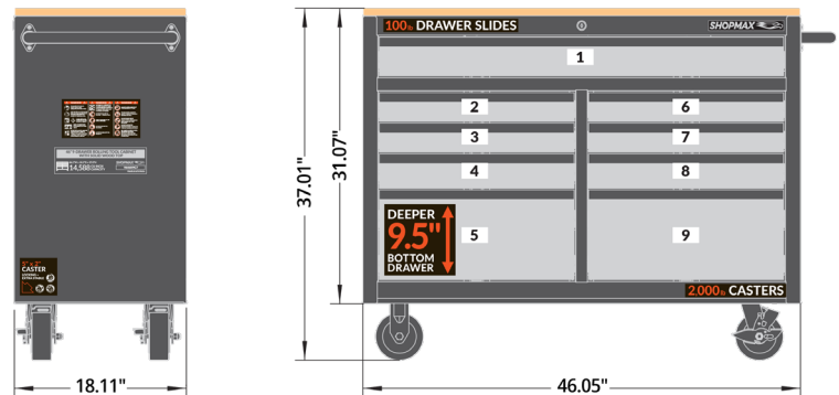
Outside dimensions and drawer numbers
