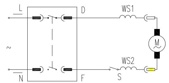
Electric circuit
