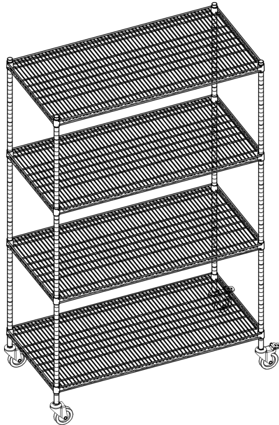
TRINITY PRO 4-TIER NSF 48" x 24" x 72" WIRE SHELVING RACK w/WHEELS Model # TBFZ-0925 / TBFPBA-0925
