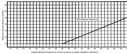
CLEARANCE REDUCTION CHART
