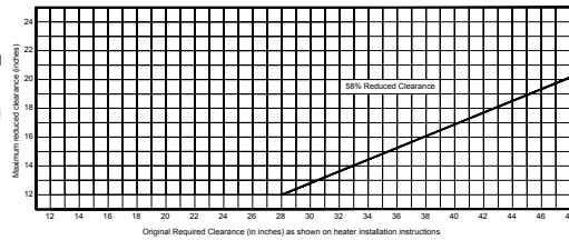
CLEARANCE REDUCTION CHART
