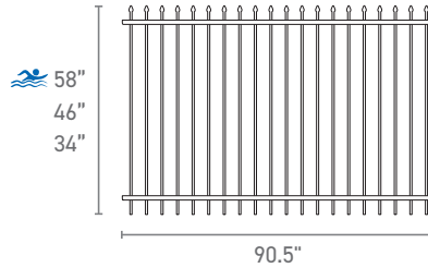
Two Rail Panels
