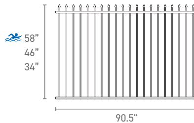
Two Rail Panels
