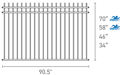
Three Rail Panels
