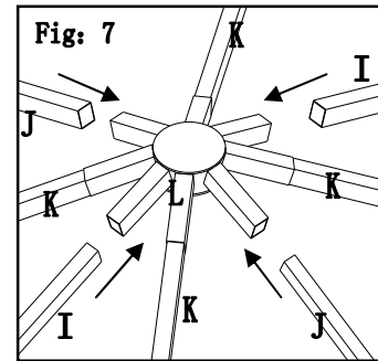
Fig.7: Insert Middle Beam (long/short) (I/J) to big top connector(L).
