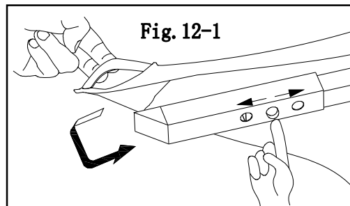
Fig.12: Fix small canopy (U1) to slanting beam (J1) (adjust tube (Y) according to the canopy size as Fig.12-1)。
