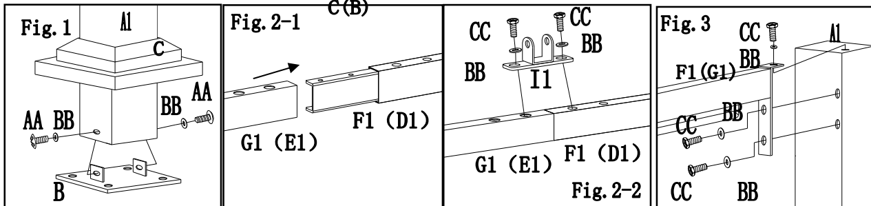
Fig.1: Put base cover (C) through bottom of post(A1), then attach base(B) to Post(A1) by using bolt(AA) and flat washer(BB).
