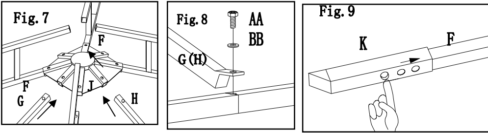
Fig.7: Insert Middle beam(G/H) to Big top connector(J).
