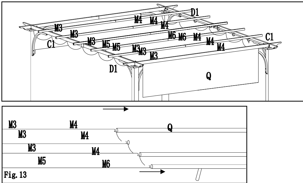
Fig.13: Insert canopy rod to the hold of canopy (Q)。(Notes: Insert canopy rod (M5、M6) to the side of handle。)
