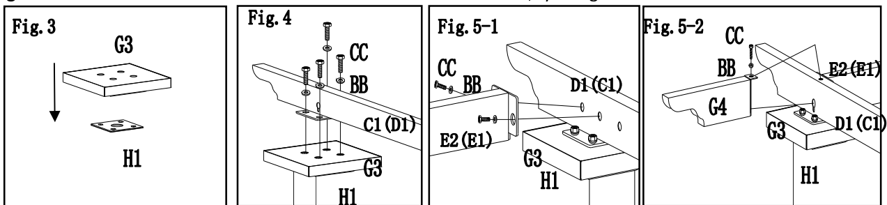
Fig.4: Attach corner (G3) to top of post (H1) .
