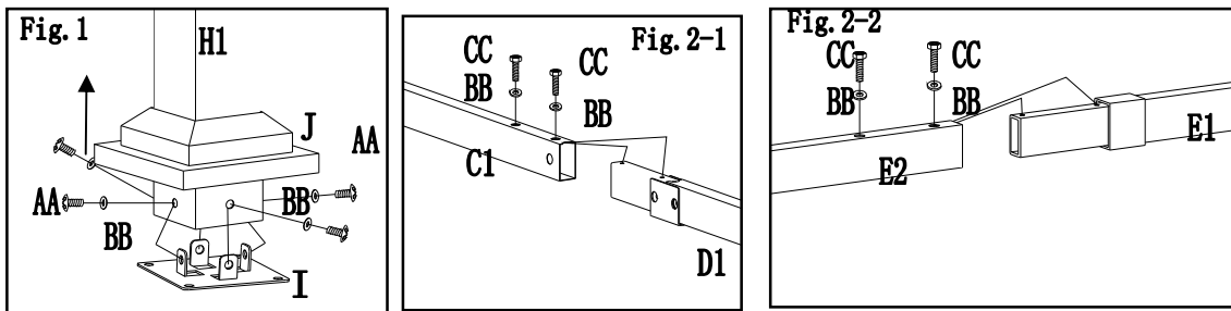
Fig.1: Put the stake cover (I) through the post (H1), up the stake cover(J), then attach stake(I) to post bottom (H1) , fasten by using bolt (AA) and washer (BB) .
