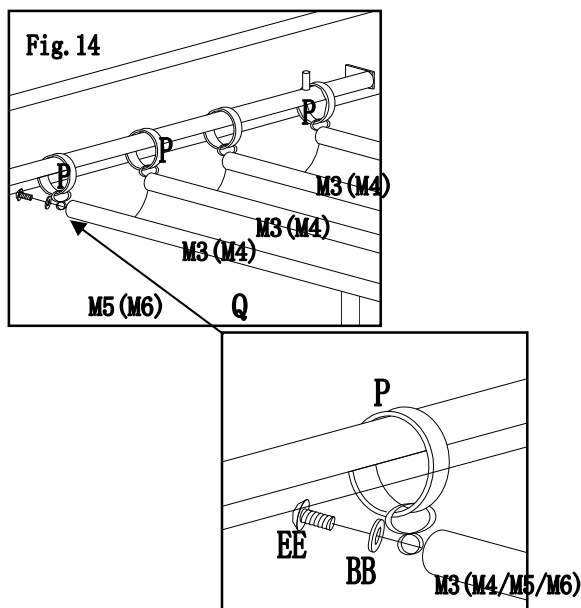
Fig.14: Fix the assembled canopy (Q) to ring (P) by using bolt (EE) and washer (BB).
