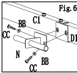
Fig.6:Attach rail connector ( N ) to long side beam ( C1、 D1 ) by using bolt ( CC ) and washer ( BB ) .
