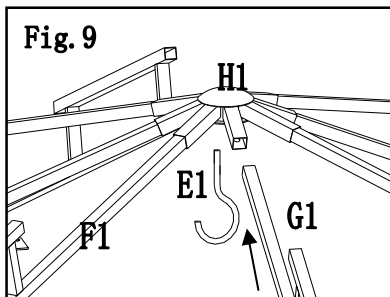
Fig.9: Insert middle beam (G1) to big top connector (H1). Then screw the hook (E1) to big top connector (H1)。
