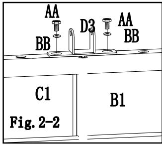
Fig.2-2: Attach middle beam lower connector(D3) to long screen(B1) and short screen(C1), by using bolt (AA)、washer (BB).
