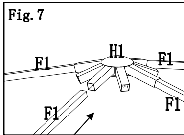
Fig.7: Insert slanting beam(F) into big top connector (H1);
