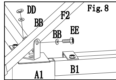
Fig.8: By using bolt (EE)、washer (BB)、nut(DD), attach slanting beam lower bar(F2) to post (A1);
