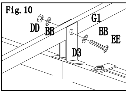
Fig.10: By using bolt (EE)、washer 片(BB)、nut (DD),attach middle beam(G1) to middle beam connector(D3);
