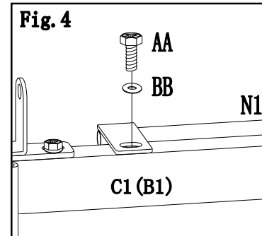
Fig.4: attach netting bar(N1)to long side screen and (B1) and short side screen (C1), by using bolt (AA)、 washer(BB).
