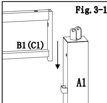
Fig.3-1: Insert the assembled screen(B1/C1) to post (A1) .
