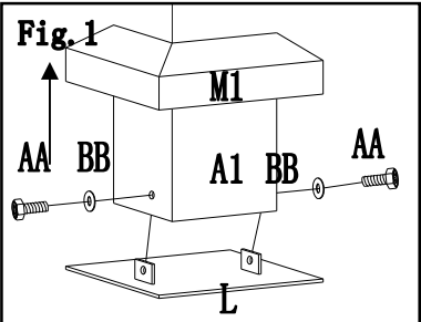
Fig.1: Put stake cover (M1) through Post(A1) and lift up stake cover, then attach stake slate (L) to bottom of post (A1) by using bolt(AA)、washer (BB).
