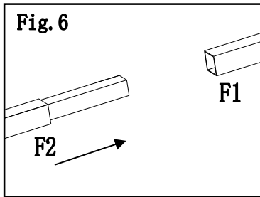
Fig.6 : Insert slanting beam lower bar(F2)into slanting beam upper bar (F1)
