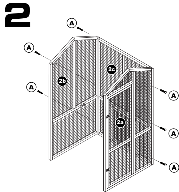
2. Connect Foraging Area Panels (2a, 2b, 2c) with Screws (A).
