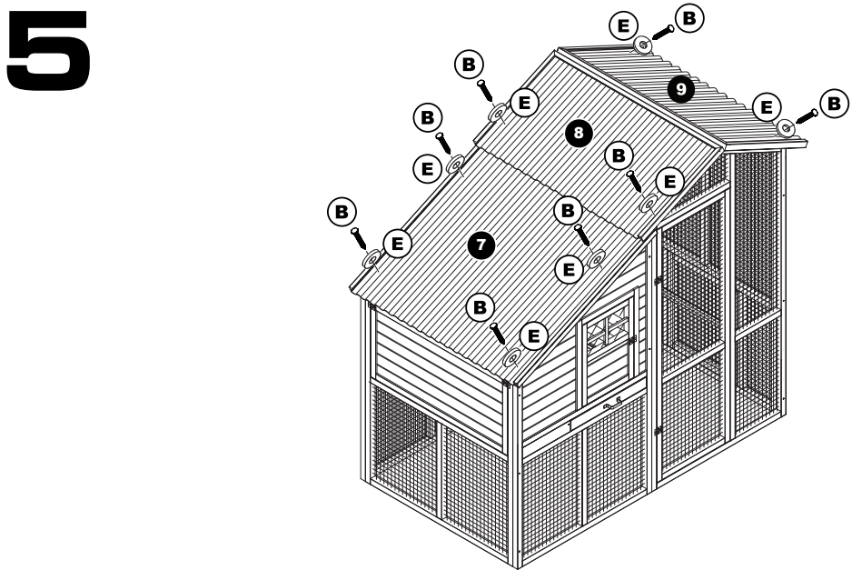
5. Attach Lower Left Roof Panel (7) with Screws (B) and Plastic Washers (E). Attach Upper Left and Right Roof Panels (8 & 9) with Screws (B) and Plastic Washers (E).
