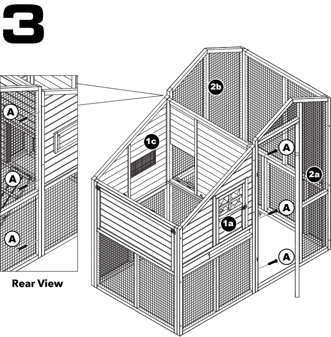
3. Connect Foraging Area Panels (2a, 2b) to Roosting Area Panels (1a, 1c) with Screws (A).
