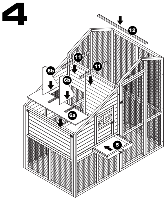
4. Insert Nesting Box Floor (6a) and Dividers (6b) into Roosting Area of coop. Insert Roosting Area Roosting Bars (11). Insert Foraging Area Roosting Bar (12). Insert Cleaning Tray (5).
