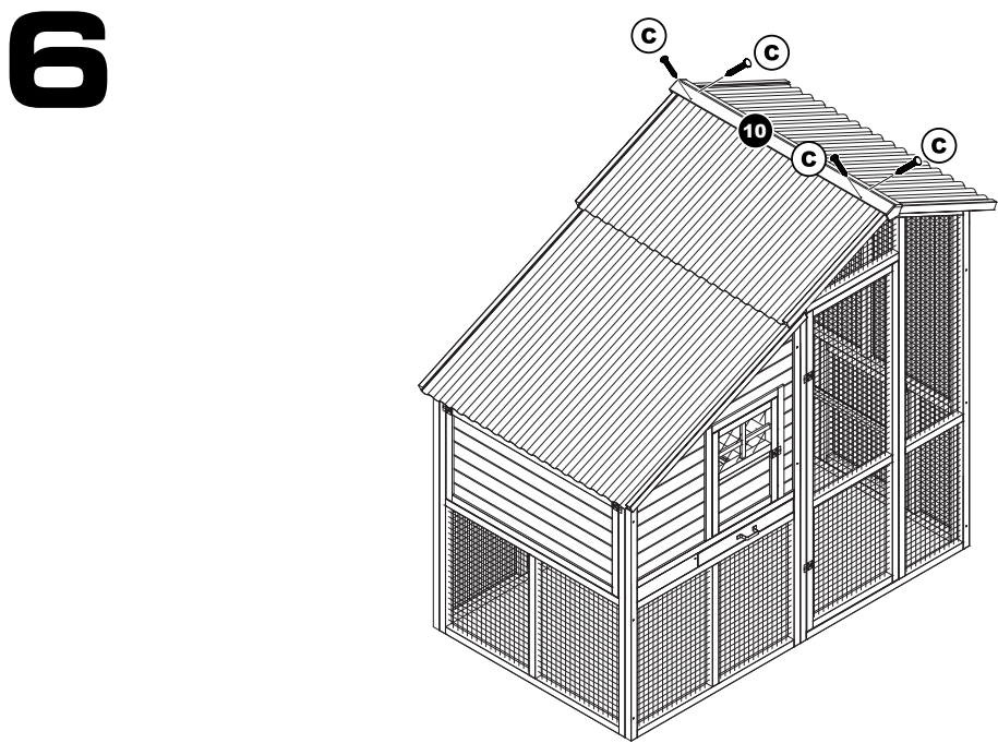
6. Attach Roof Cap (10) with Screws (C).
