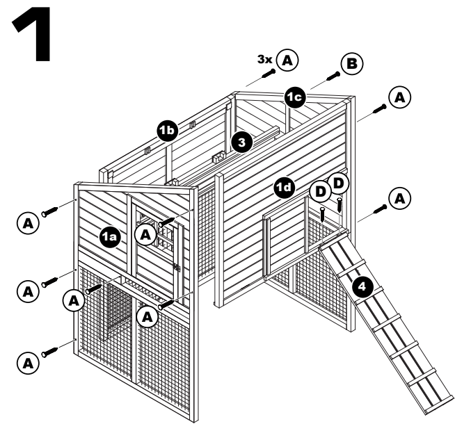
1. Connect Roosting Area Panels (1a, 1b, 1c, 1d) with Screws (A). Attach Nesting Box Floor Support (3) with Screws (A-On Front, B-On Back). Attach Ramp (4) with Screws (D).
