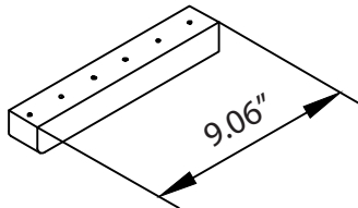
15 TABLE TOP END STRETCHER X2PCS
